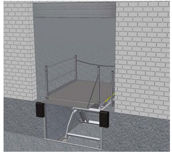
(B) Interior Grade Level To Higher Dock Level Full Pit Installation (Pit Mount)
